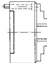
A09 Duro-M - 3-Jaws, drilling and turning jaws, cylindrical center mount, mounting from front, (DIN 6350 modified)
