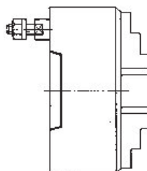
A09 Duro-M - 3-Jaws, Base and top jaws, With studs and locknuts (ISO 702-3/DIN 55027)
