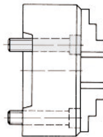
A09 Duro-M - 4-Jaws, Base and top jaws, Short taper mount, mounting from front (ISO 702-1/DIN 55026)
