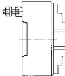
A09 Duro-M - 4-Jaws, Base and top jaws, With studs and locknuts (ISO 702-3/DIN 55027)
